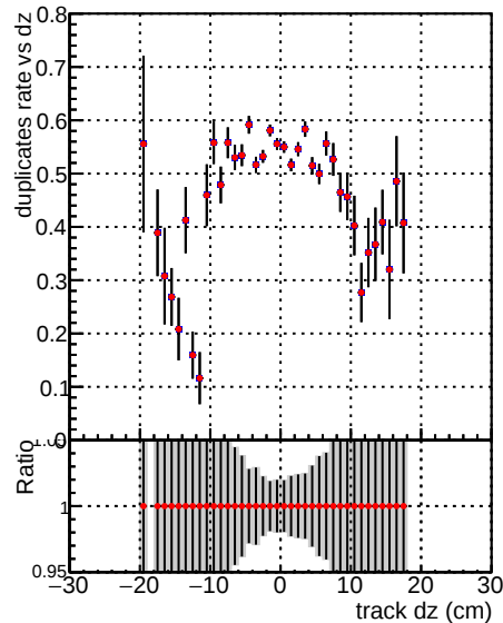
—●— DQM_V0001_R0000000001_Global_mkFit_nobatch —●— DQM_V0001_R0000000001_Global_mkFit_maybebatch
