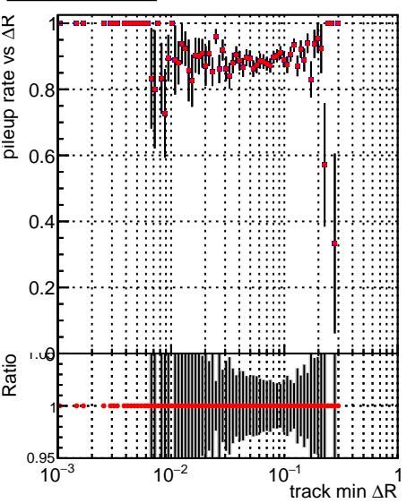
—●— DQM_V0001_R000000001_Global_mkFit_nobatch —●— DQM_V0001_R000000001_Global_mkFit_maybebatch
