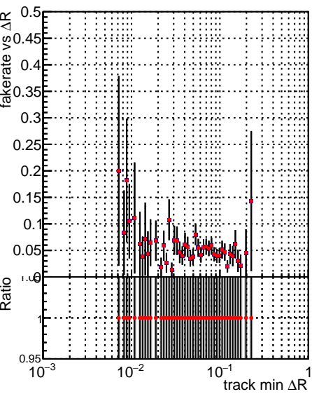
—●— DQM_V0001_R000000001_Global_mkFit_nobatch —●— DQM_V0001_R000000001_Global_mkFit_maybebatch
