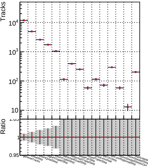
DQM_V0001_R0000000001_Global_mkFit_nobatch
