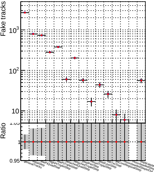
Number ● DQM_V0001_R0000000001_Global_mkFit_maybebatch
