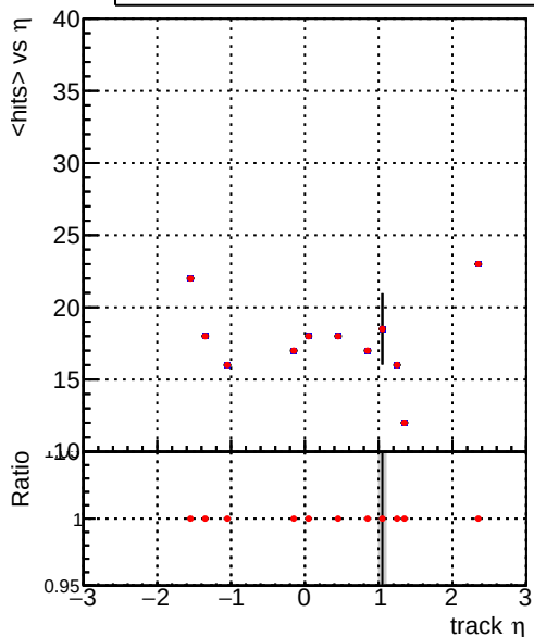
mean hits vs \eta Legend: DQM_V0001_R000000001_Global_mkFit_nobatch (blue line), DQM_V0001_R000000001_Global_mkFit_maybebatch (red line)
