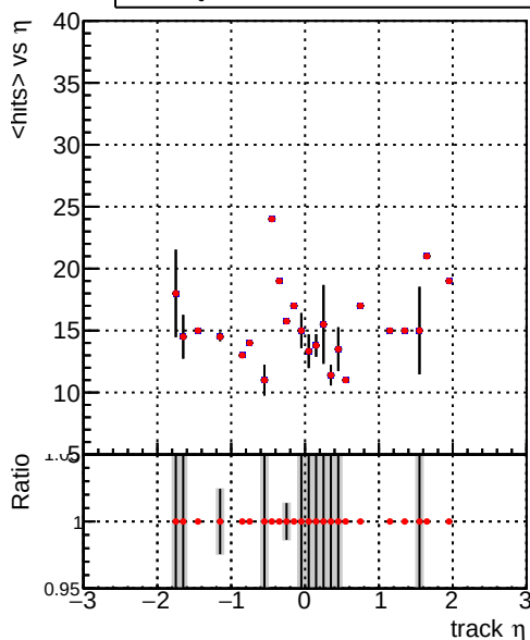
— DQM_V0001_R000000001_Global_mkFit_nobatch — DQM_V0001_R000000001_Global_mkFit_maybebatch
