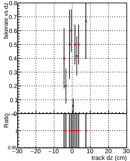
Fake rate vs dz Legend: Black line with blue dots: DQM_V0001_R0000000001 Global mkFit nobatch Red line with red dots: DQM_V0001_R0000000001 Global mkFit maybebatch
