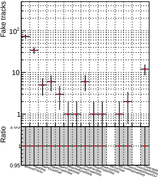
Number ● DQM_V0001_R000000001_Global_mkFit_maybebatch
