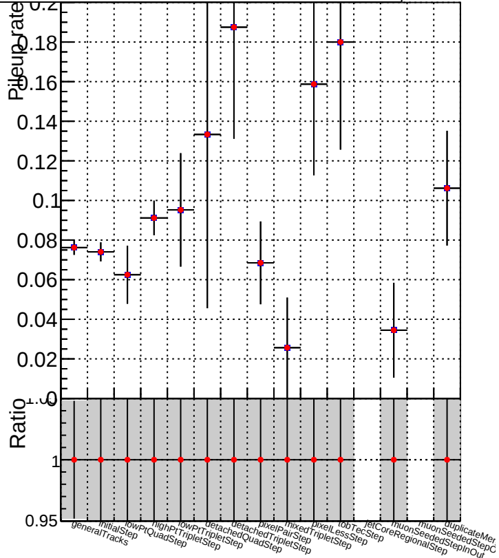
DQM_V0001_R000000001_Global_mkFit_nobatch DQM_V0001_R000000001_Global_mkFit_maybebatch
