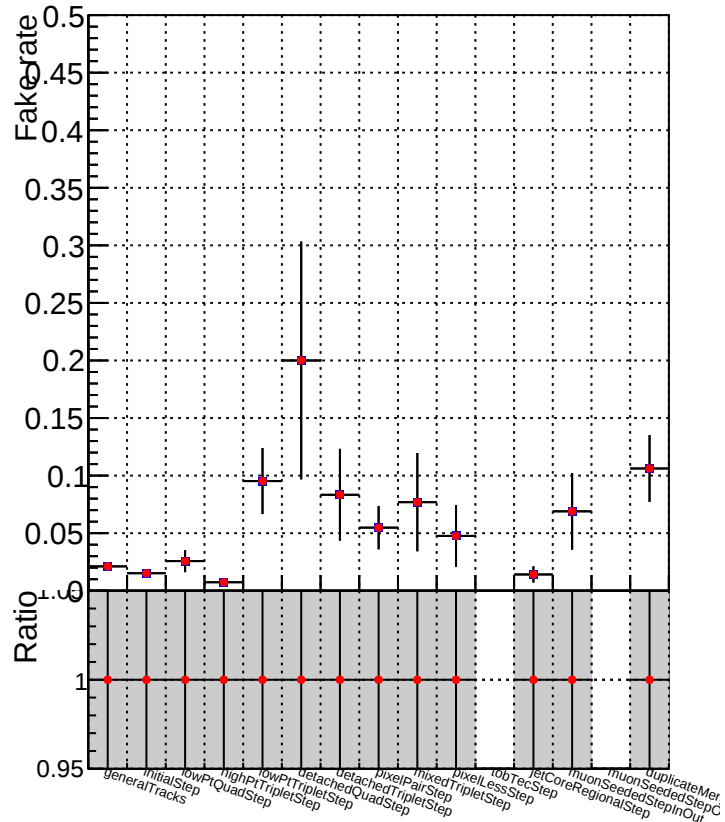
DQM_V0001_R000000001_Global_mkFit_nobatch DQM_V0001_R000000001_Global_mkFit_maybebatch
