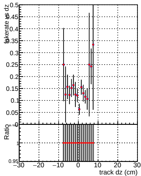
Fake rate vs dz —●— DQM_V0001_R0000000001_Global_mkFit_nobatch —●— DQM_V0001_R0000000001_Global_mkFit_maybebatch
