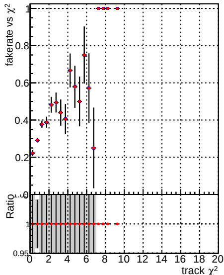
Fake rate vs. —•— DQM_V0001_R0000000001_Global_mkFit_nobatch —•— DQM_V0001_R0000000001_Global_mkFit_maybebatch
