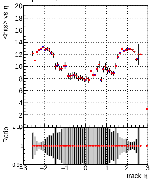
— DQM_V0001_R000000001_Global_mkFit_nobatch — DQM_V0001_R000000001_Global_mkFit_maybebatch
