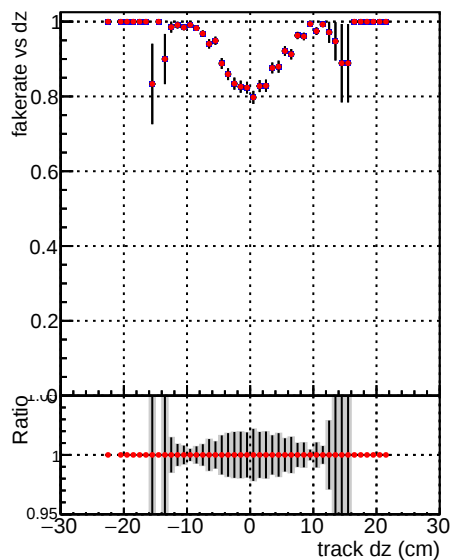
Fake rate vs dz Legend: Global mkFit nobatch (black line with blue dots) Global mkFit maybepatch (red line with red dots)
