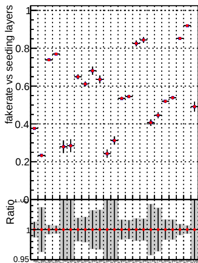
Fake rate vs. Legend Global mkFit nobatch Blue star DQM_V0001_R0000000001 Red star DQM_V0001_R0000000001 mkFit maybebatch
