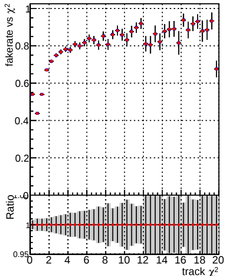
Fake rate vs. Legend Global mkFit nobatch Blue star DQM_V0001_R0000000001 Red star DQM_V0001_R0000000001 mkFit maybebatch
