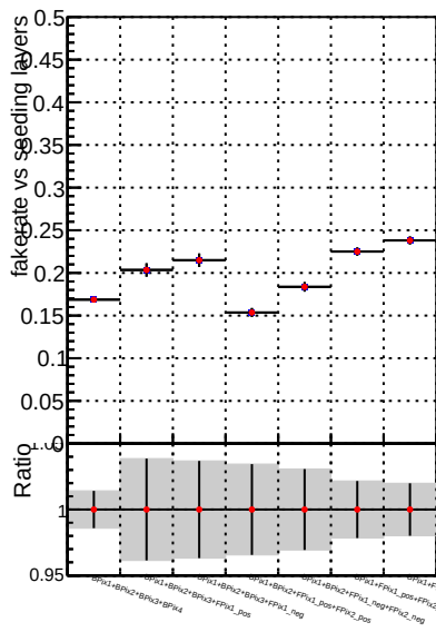
Fake rate vs. Legend Global mkFit nobatch Blue line with dots DQM V0001_R000000001 Red line with dots DQM V0001_R000000001 mkFit maybebatch
