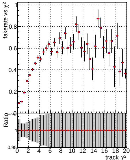
Fake rate vs. Legend Global mkFit nobatch Blue line with dots DQM V0001_R000000001 Red line with dots DQM V0001_R000000001 mkFit maybebatch
