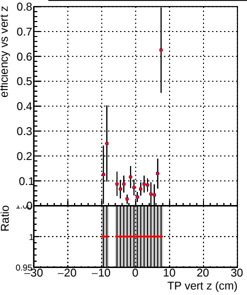
Efficiency vs vert z Legend: DQM_V0001_R000000001_Global_mkFit_nobatch DQM_V0001_R000000001_Global_mkFit_maybebatch
