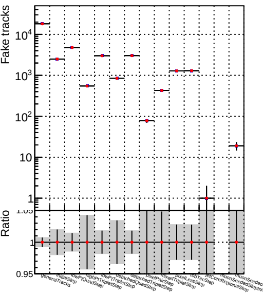
Number ● DQM_V0001_R0000000001_Global_mkFit_maybebatch
