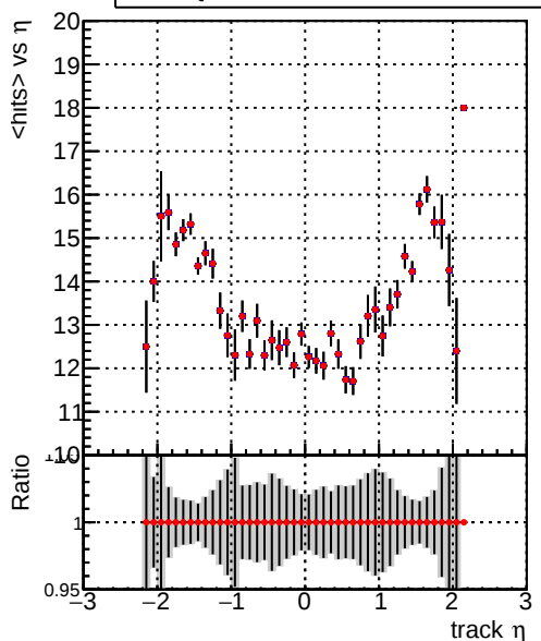
— DQM_V0001_R000000001_Global_mkFit_nobatch — DQM_V0001_R000000001_Global_mkFit_maybepoch
