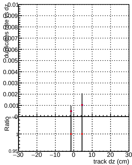
—•— DQM V0001_R000000001 Global mkFit nobatch —•— DQM V0001_R000000001 Global mkFit maybebatch
