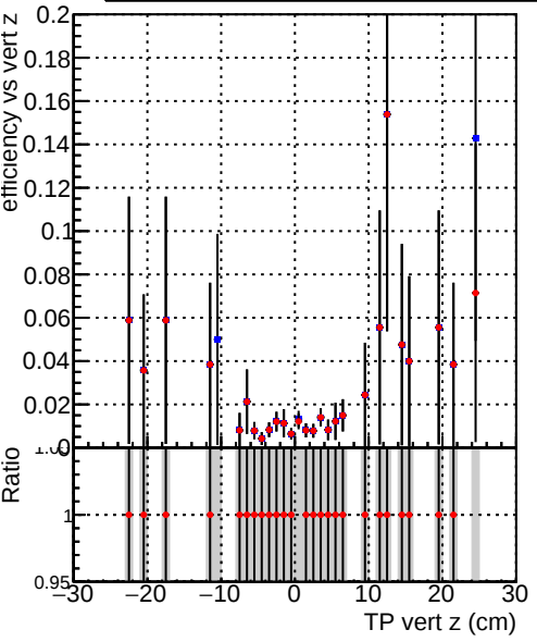
Efficiency vs TP vert z (cm) Legend: DQM_V0001_R0000000001_Global_mkFit_batch DQM_V0001_R0000000001_Global_mkFit_NObatch
