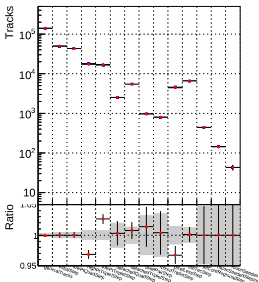
DQM_V0001_R000000001_Global_mkFit_batch
