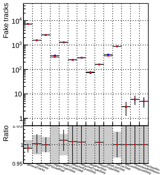
Number —●— DQM_V0001_R000000001_Global_mkFit_NObatch
