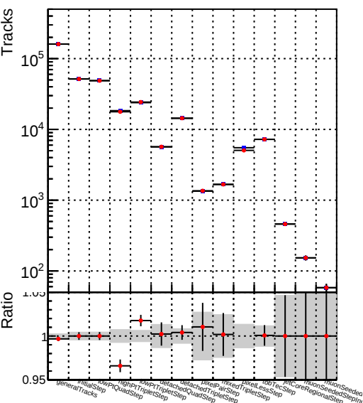
DQM_V0001_R000000001__Global__mkFit_batch
