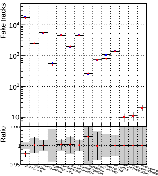
Number —●— DQM_V0001_R0000000001_Global_mkFit_NObatch
