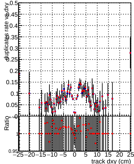
—●— DQM_V0001_R000000001_Global_mkFit_batch —●— DQM_V0001_R000000001_Global_mkFit_NObatch
