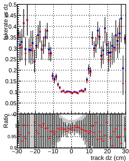
—●— DQM_V0001_R000000001_Global_mkFit_batch —●— DQM_V0001_R000000001_Global_mkFit_NObatch
