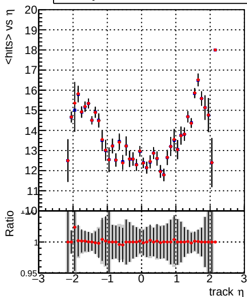
— DQM_V0001_R000000001_Global_mkFit_batch — DQM_V0001_R000000001_Global_mkFit_NObatch
