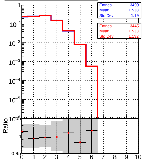
mean hit — DQM_V0001_R000000001_Global_mkFit_batch — DQM_V0001_R000000001_Global_mkFit_NObatch
