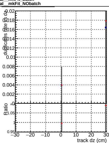
—●— DQM V0001_R000000001 Global mkFit batch —●— DQM V0001_R000000001 Global mkFit NObatch
