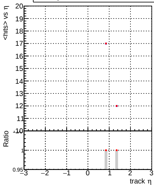
— DQM_V0001_R000000001_Global_mkFit_batch — DQM_V0001_R000000001_Global_mkFit_NObatch
