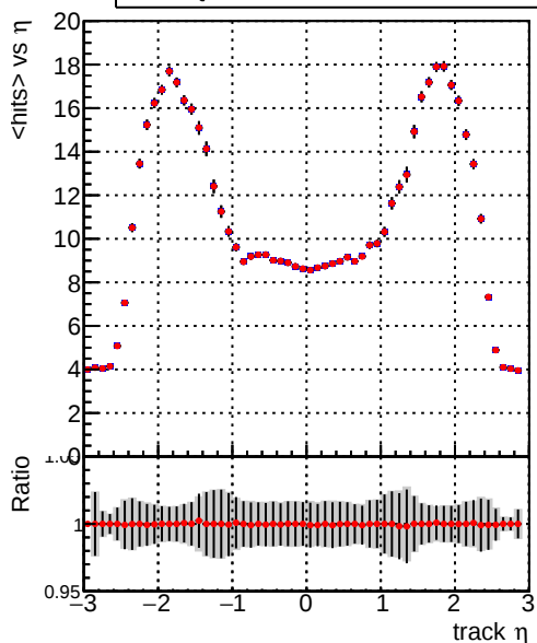
mean hits vs \eta Legend: DQM_V0001_R000000001_Global_mkFit_batch (blue line), DQM_V0001_R000000001_Global_mkFit_NObatch (red line)
