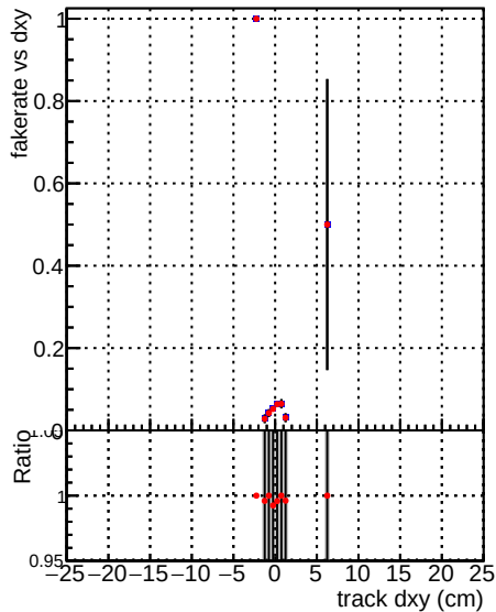
Fake rate vs d DQM_V0001_R000000001 Global mkFit batch DQM_V0001_R000000001 Global mkFit NObatch
