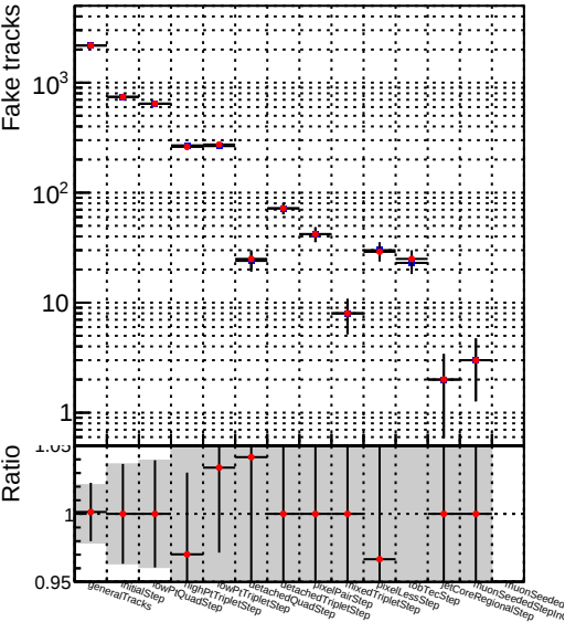
Number —●— DQM_V0001_R000000001_Global_mkFit_NObatch
