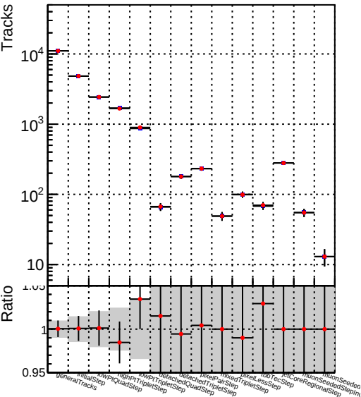
DQM_V0001_R000000001__Global__mkFit_batch
