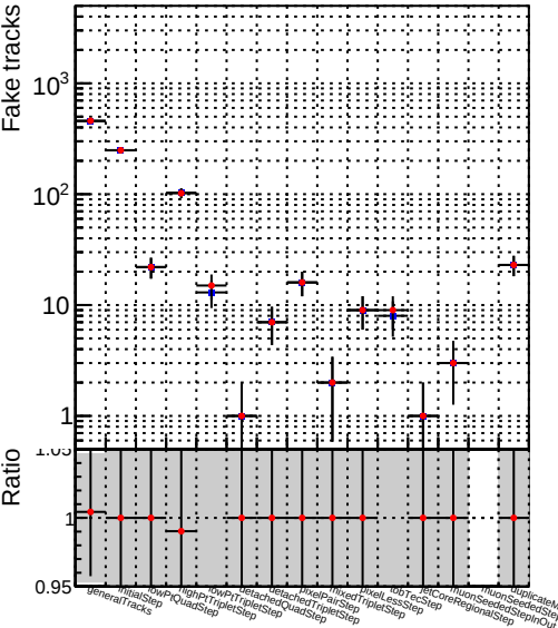
Number —●— DQM_V0001_R000000001_Global_mkFit_NObatch
