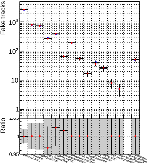
Number —●— DQM_V0001_R0000000001_Global_mkFit_NObatch
