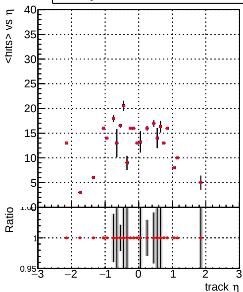
mean hit — DQM_V0001_R000000001_Global_mkFit_batch — DQM_V0001_R000000001_Global_mkFit_NObatch
