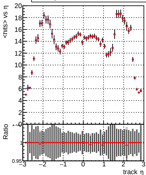
mean hit Legend: DQM_V0001_R000000001_Global_mkFit_batch (blue line with dots), DQM_V0001_R000000001_Global_mkFit_NObatch (red line with dots)
