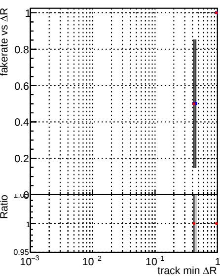
Fake rate vs ΔR(track, jet) DQM_V0001_R000000001_Global_mkFit_batch DQM_V0001_R000000001_Global_mkFit_NObatch
