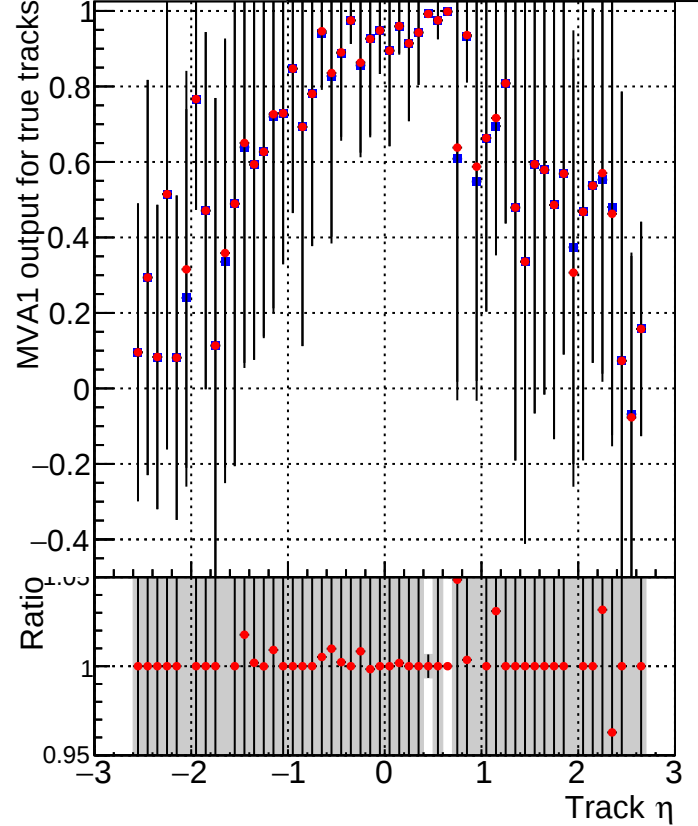
MVA1 of associated tracks (recoToSim) vs. track \eta Legend: ■ DQM_V0001_R000000001_Global_mkFit_batch ● DQM_V0001_R000000001_Global_mkFit_NObatch
