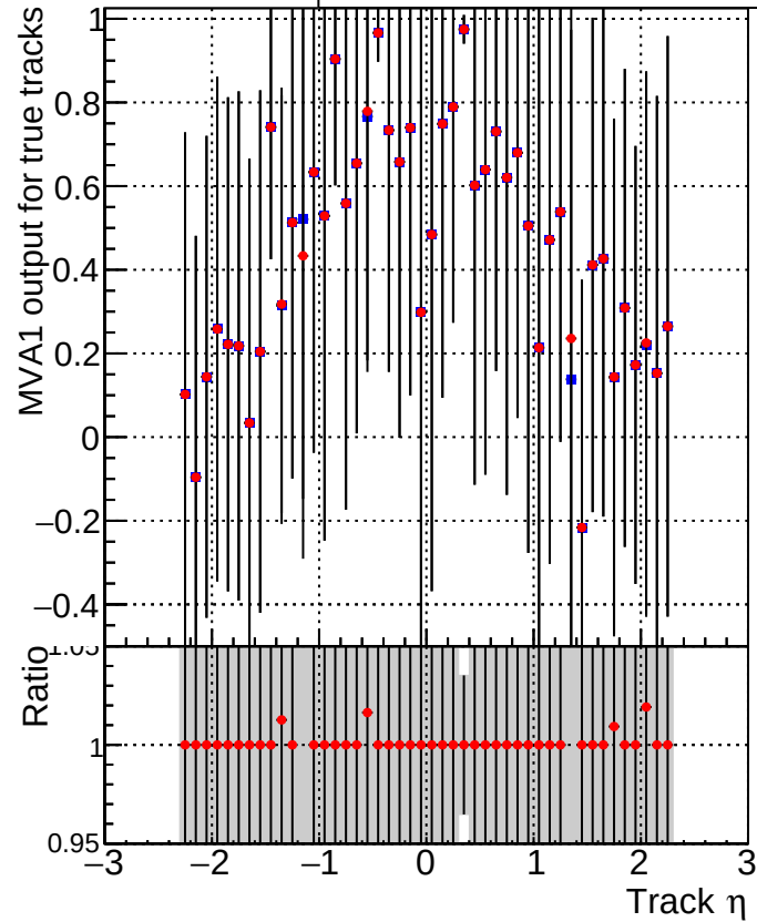
MVA1 of associated tracks (recoToSim) vs. track \eta Legend: ■ DQM_V0001_R000000001_Global_mkFit_batch ● DQM_V0001_R000000001_Global_mkFit_NObatch
