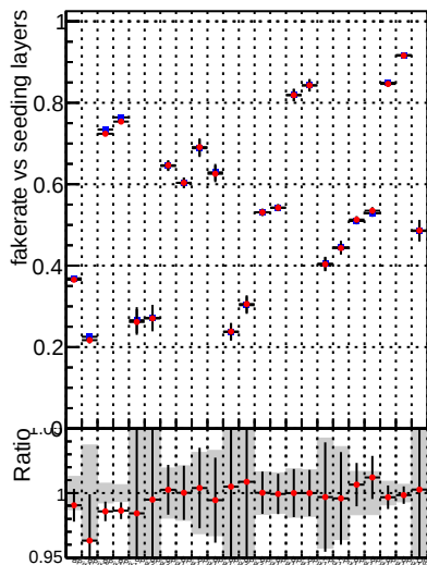
Fake rate vs. —•— DQM V0001_R000000001 Global mkFit batch —•— DQM V0001_R000000001 Global mkFit NObatch
