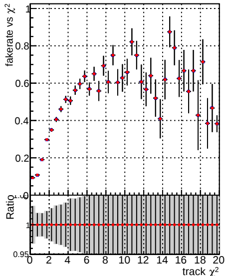
Fake rate vs. —•— DQM_V0001_R000000001_Global_mkFit_batch —•— DQM_V0001_R000000001_Global_mkFit_NObatch
