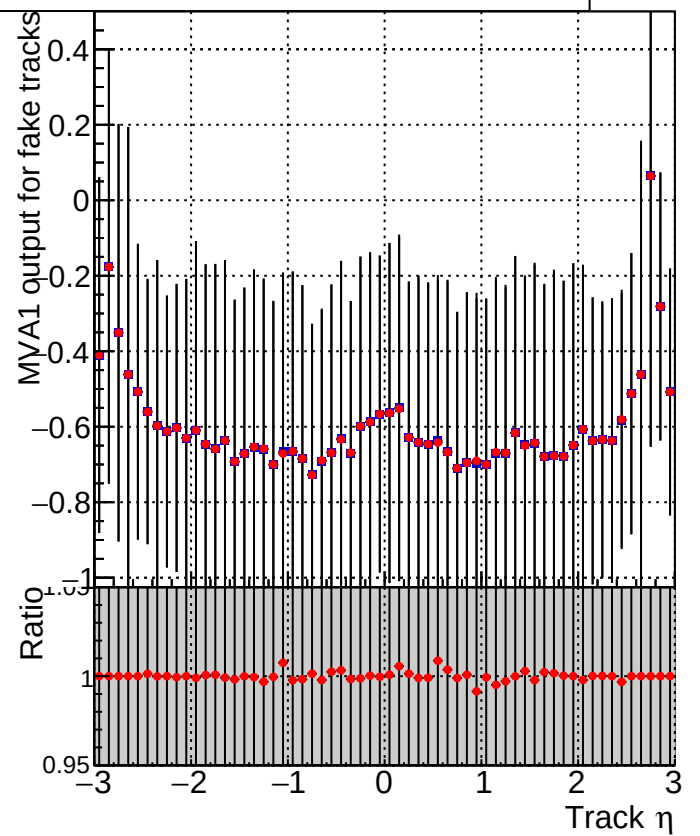
MVA1 of associated tracks (recoToSim) vs. track \eta Legend: ■ DQM_V0001_R0000000001_Global_mkFit_batch ■ DQM_V0001_R0000000001_Global_mkFit_NObatch
