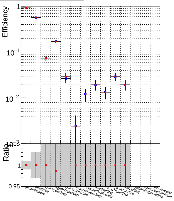
DQM_V0001_R000000001_Global_mkFit_batch DQM_V0001_R000000001_Global_mkFit_NObatch
