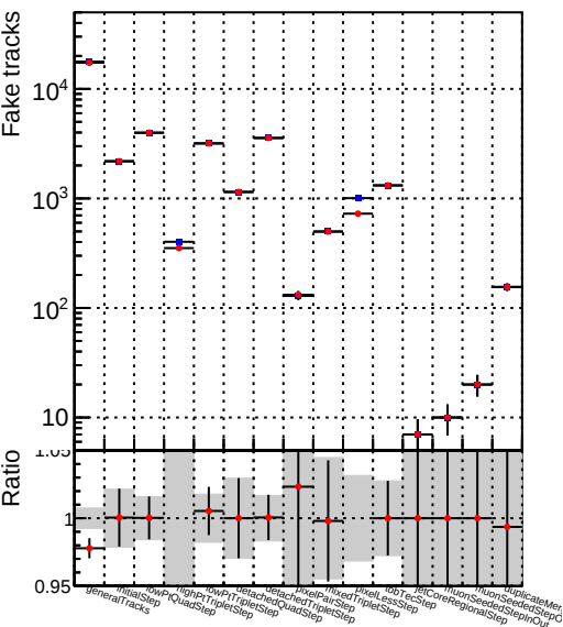
Number —●— DQM_V0001_R000000001_Global_mkFit_NObatch
