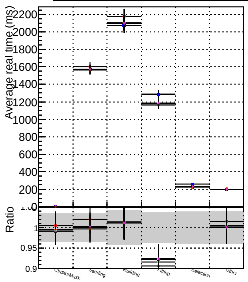
Average DOM V0001 R0000000001 Global mkFit Noval DOM V0001 R0000000001 Global mkFit batch DOM V0001 R0000000001 Global mkFit batch32 DOM V0001 R0000000001 Global mkFit batch64
