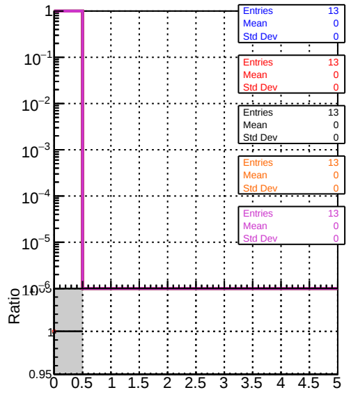
mean hit DOM V0001 R0000000001 Global mkFit NoEval DOM V0001 R0000000001 Global mkFit batch DOM V0001 R0000000001 Global mkFit batch32 DOM V0001 R0000000001 Global mkFit batch64
