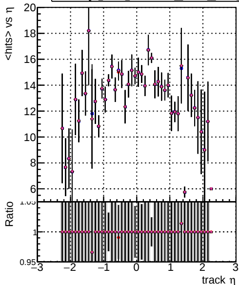
mean hit DOM V0001 R0000000001 Global mkFit NoEval DOM V0001 R0000000001 Global mkFit batch DOM V0001 R0000000001 Global mkFit batch32 DOM V0001 R0000000001 Global mkFit batch64
