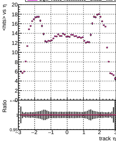
Legend for mean hits vs track \eta : DOM V0001 R0000000001 Global mkFit NoEval DOM V0001 R0000000001 Global mkFit batch DOM V0001 R0000000001 Global mkFit batch32 DOM V0001 R0000000001 Global mkFit batch64
