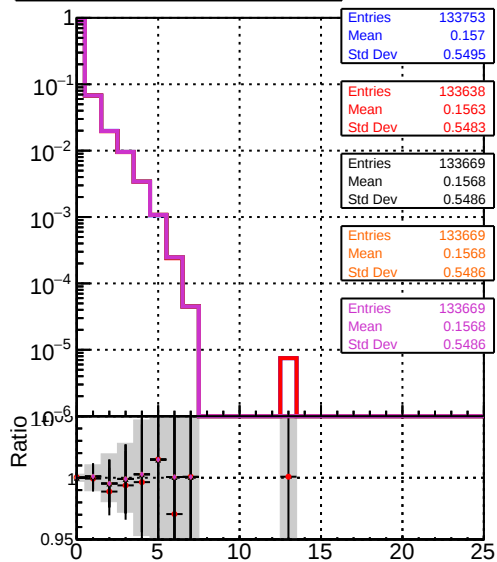
Legend: DOM V0001 R0000000001 Global mkFit NoEval, DOM V0001 R0000000001 Global mkFit batch, DOM V0001 R0000000001 Global mkFit batch32, DOM V0001 R0000000001 Global mkFit batch64 mean hits
