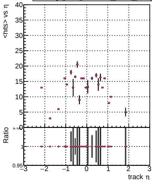
mean hits DOM V0001 R0000000001 Global mkFit NoEval DOM V0001 R0000000001 Global mkFit NoBatch DOM V0001 R0000000001 Global mkFit batch DOM V0001 R0000000001 Global mkFit batch32 DOM V0001 R0000000001 Global mkFit batch64
