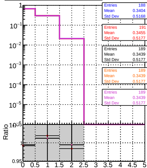
mean hits vs \eta DOM V0001 R0000000001 Global mkFit NoEval DOM V0001 R0000000001 Global mkFit batch DOM V0001 R0000000001 Global mkFit batch32 DOM V0001 R0000000001 Global mkFit batch64
