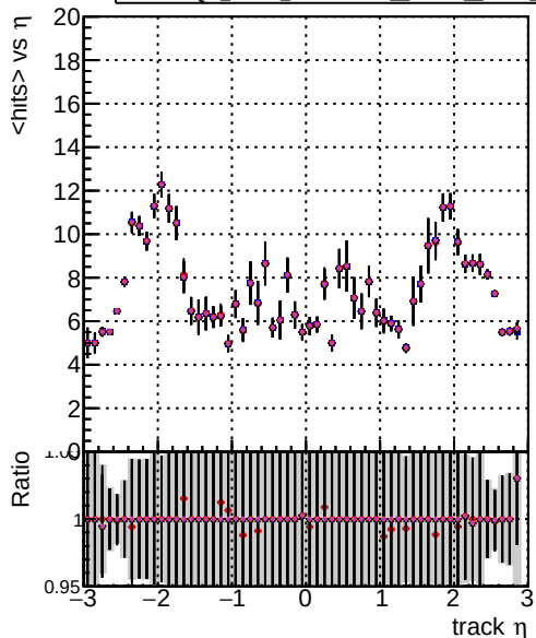
Legend for mean hits vs track \eta : DOM V0001 R0000000001 Global mkFit NoEval DOM V0001 R0000000001 Global mkFit batch DOM V0001 R0000000001 Global mkFit batch32 DOM V0001 R0000000001 Global mkFit batch64
