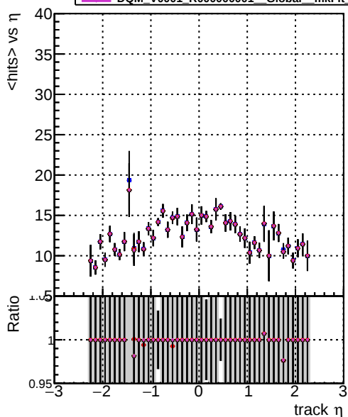
mean hit DOM V0001 R000000001 Global mkFit NoEval DOM V0001 R000000001 Global mkFit batch DOM V0001 R000000001 Global mkFit batch32 DOM V0001 R000000001 Global mkFit batch64
